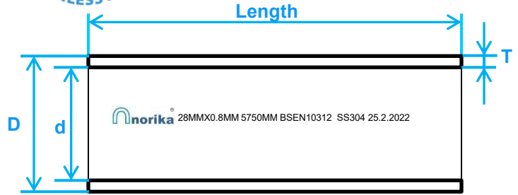
CROSS SECTION VIEW
