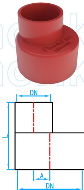
SIDE VIEW
