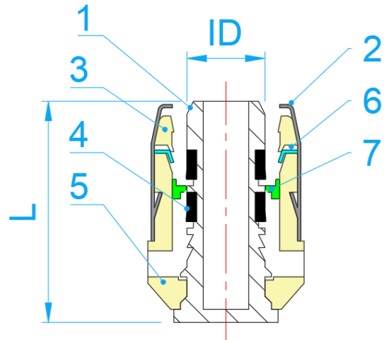
SECTION VIEW
