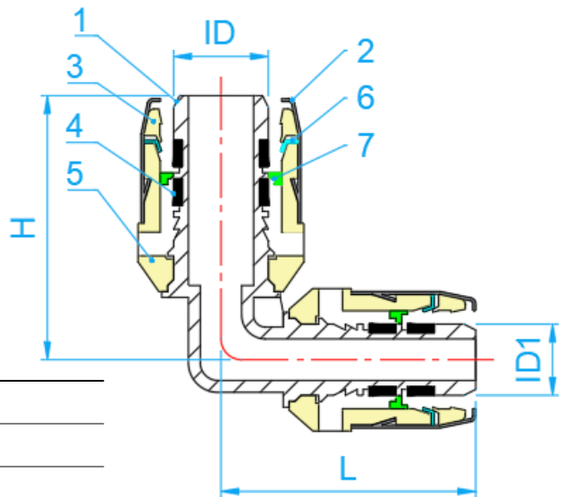
SECTION VIEW
