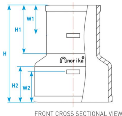
FRONT CROSS SECTIONAL VIEW
