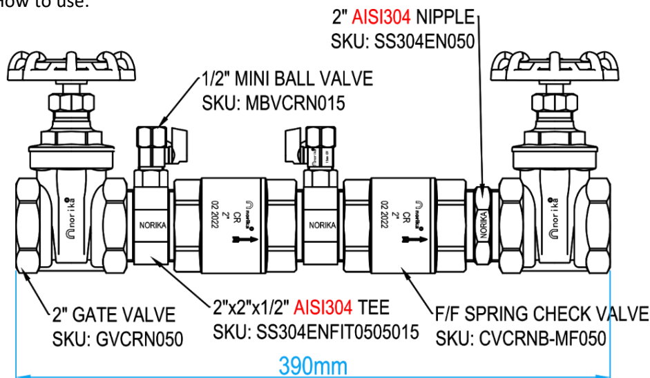
NORIKA MODIFIED DESIGN Second Generation
