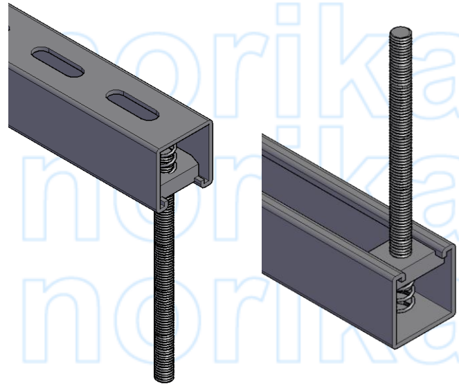
INSTALLATION ASSEMBLY
