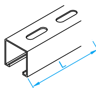
3-D VIEW
