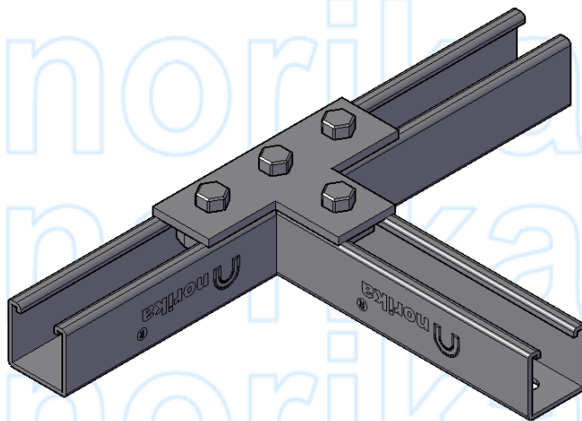
INSTALLATION ASSEMBLY
