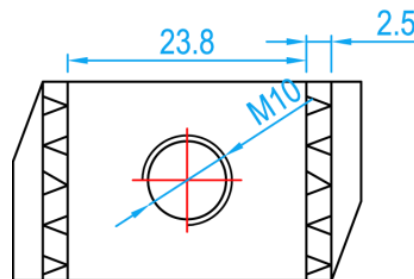
BOTOM VIEW
