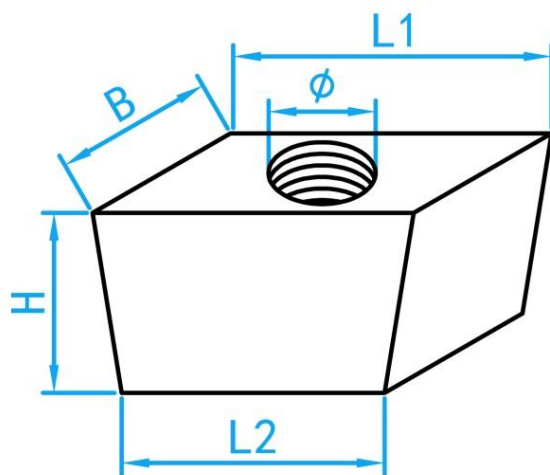
3D View
