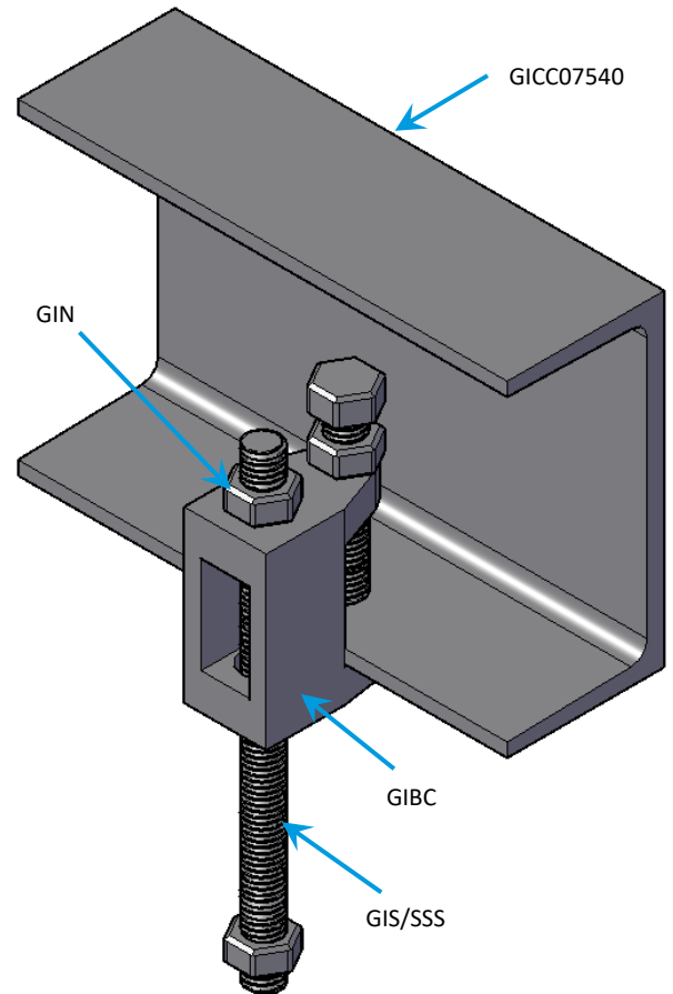
INSTALLATION ASSEMBLY
