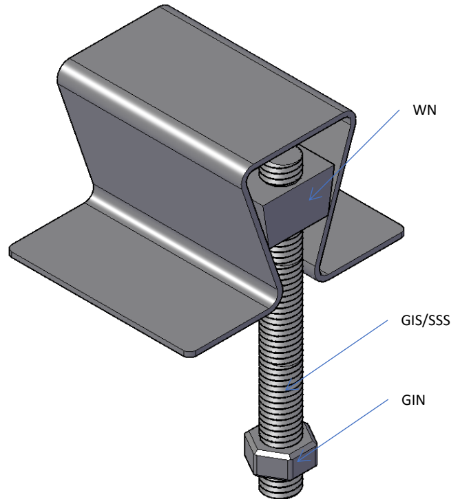
INSTALLATION ASSEMBLY
