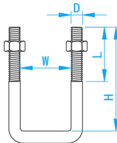
U BOLT SIDE VIEW
