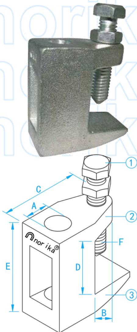
3-D VIEW
