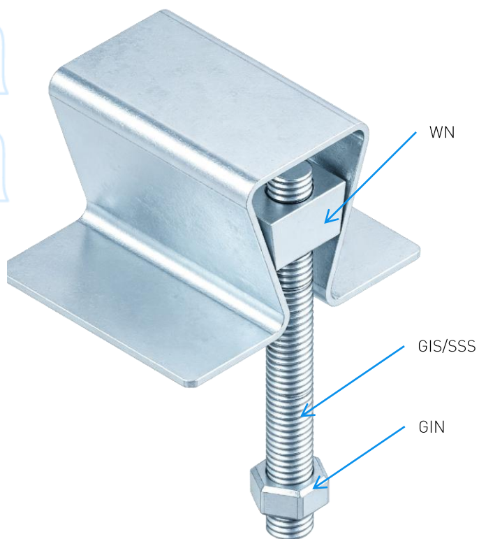
INSTALLATION ASSEMBLY
