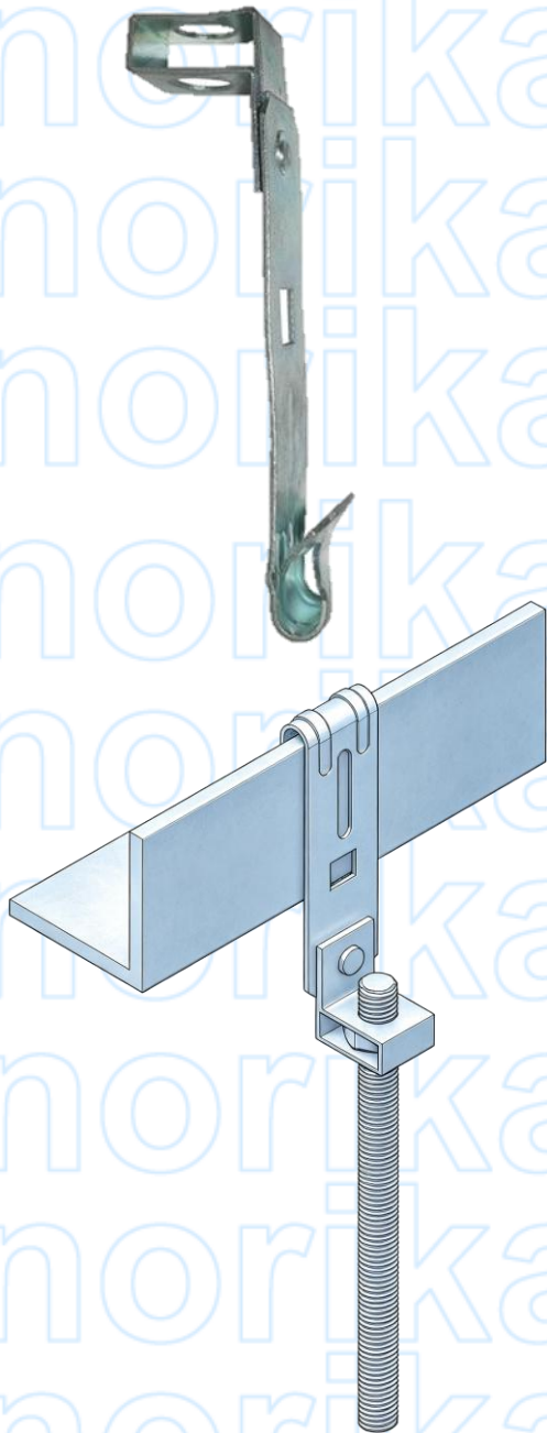
INSTALLATION ASSEMBLY
