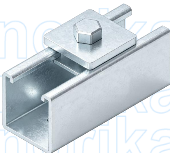
INSTALLATION ASSEMBLY
