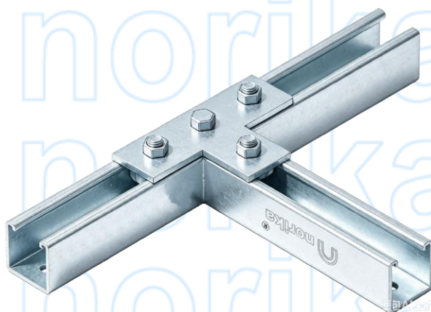
INSTALLATION ASSEMBLY
