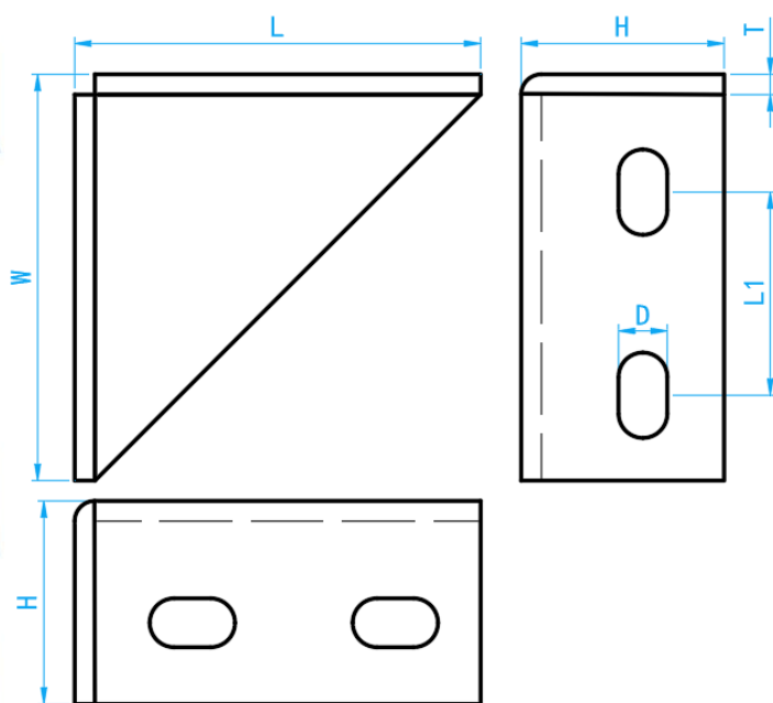
SIDE VIEW
