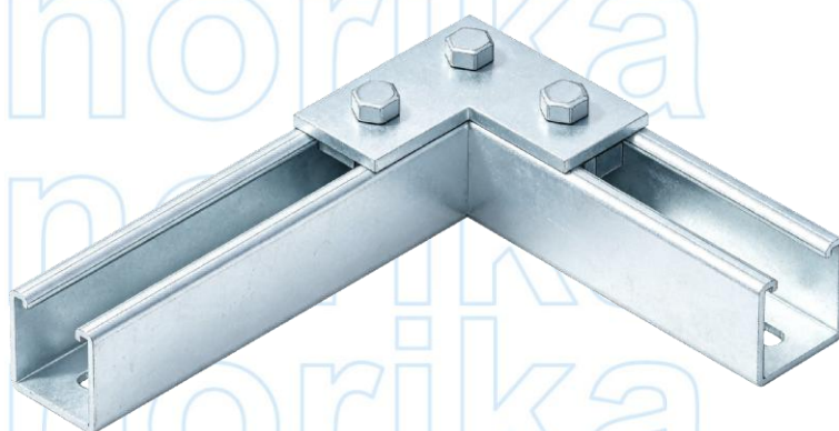
INSTALLATION ASSEMBLY
