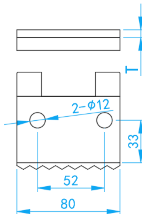
PRESSPLATE TOP VIEW
