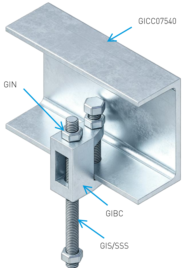
INSTALLATION ASSEMBLY
