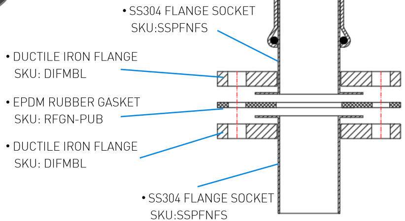
INSTALLATION ASSEMBLY
