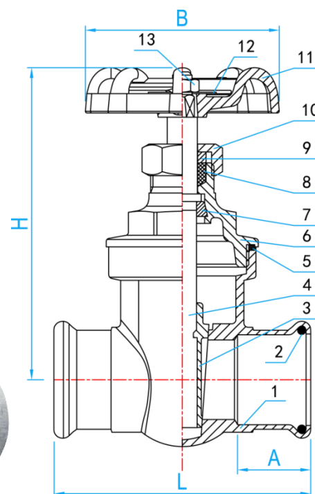
CROSS SECTIONAL VIEW
