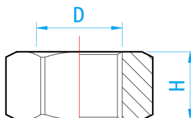
SECTIONAL VIEW
