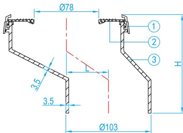
SECTION VIEW
