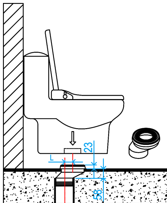
SECTION VIEW
