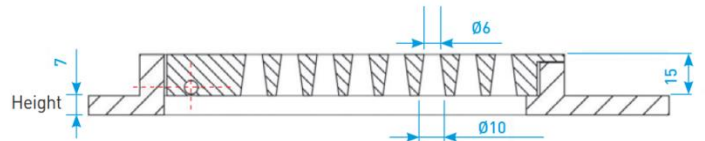
SECTION C-C
