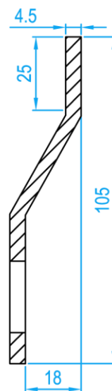
SIDE SECTION VIEW
