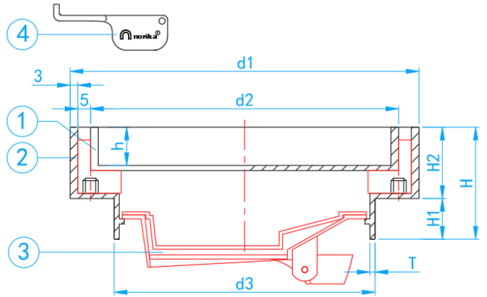
CROSS SECTIONAL VIEW
