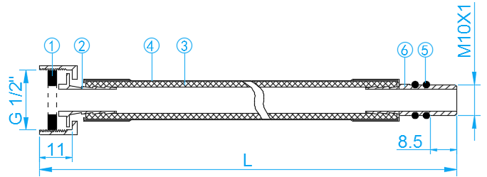
SECTION VIEW
