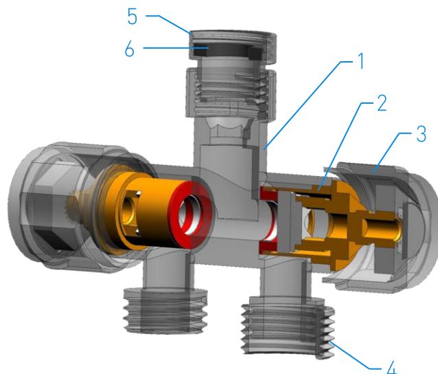
SECTION VIEW
