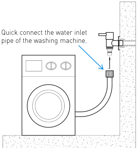
INSTALLATION ASSEMBLY
