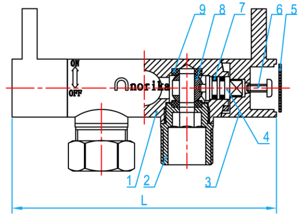
SECTION VIEW
