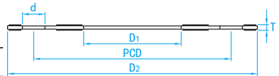
CROSS SECTIONAL VIEW
