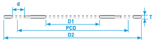
CROSS SECTIONAL VIEW
