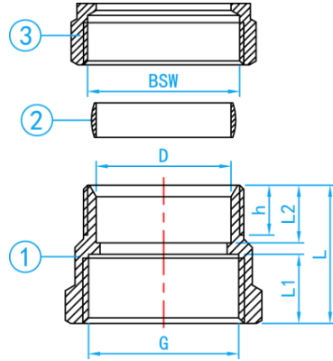
SECTION VIEW
