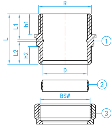
SECTION VIEW
