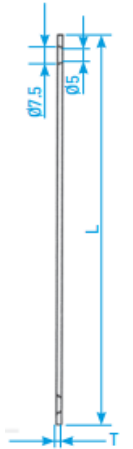
CROSS SECTIONAL VIEW
