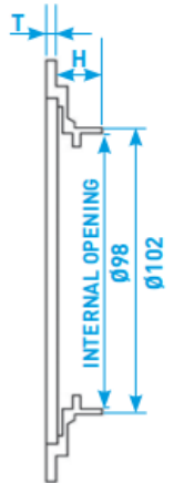
CROSS SECTIONAL VIEW
