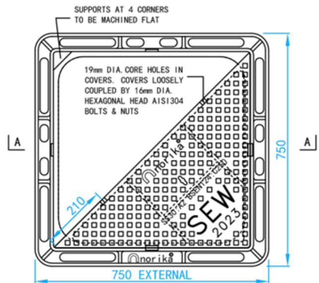
HALF COVER REMOVED TOP VIEW
