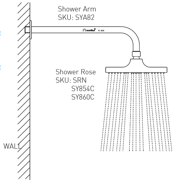
INSTALLATION ASSEMBLY
