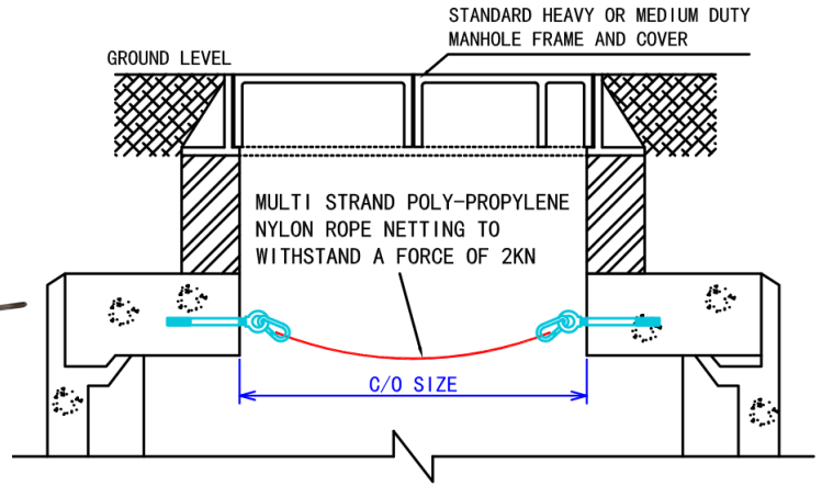
SECTION VIEW
