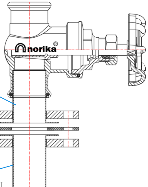
INSTALLATION ASSEMBLY
