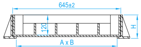
SECTION VIEW
