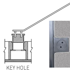
KEY HOLE
