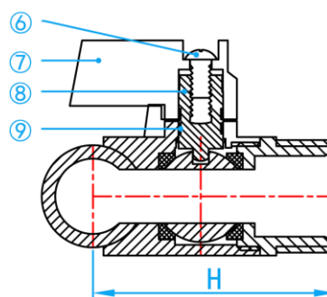
CROSS SECTIONAL VIEW
