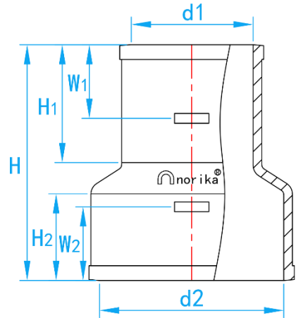
FRONT SECTIONAL VIEW
